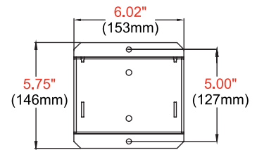
WALL PLATE DETAIL
