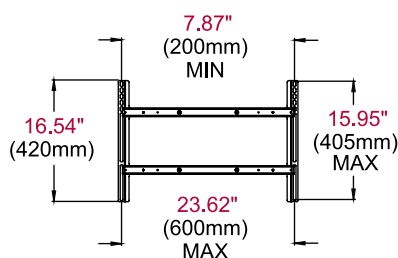
ADAPTOR PLATE
